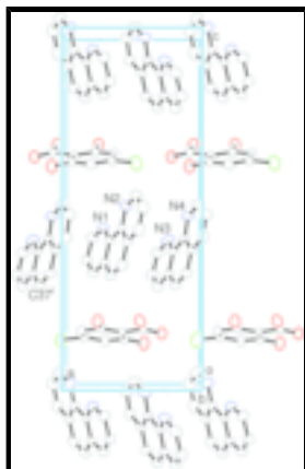
Fig. 2. A packing diagram for (I) showing \pi - \pi stacking between phen and Hphen ring systems [symmetry code: (i) 1 + x, y, z ]. The H atoms are omitted for clarity.
